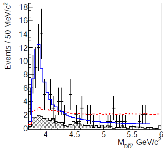
Fig. 1. Projections of the signal fit results in the default model onto M_{D\bar{D}} . The points with error bars are the data, the hatched histograms are the background, the blue solid line is the fit with a new X^* resonance ( J^{PC} = 0^{++} ) and the red dashed line is the fit with nonresonant amplitude only.
