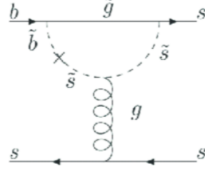
Figure 4: Example of Feynman diagram for a gluonic penguin b \rightarrow sq\bar{q} decay.
