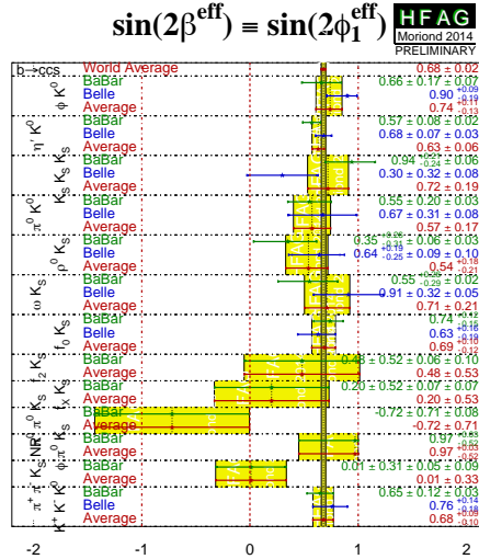
Figure 5: Compilation of results for \sin(2\beta^{\text{eff}}) \equiv \sin(2\phi_1^{\text{eff}}) for several b \rightarrow sq\bar{q} decay modes from [5].
