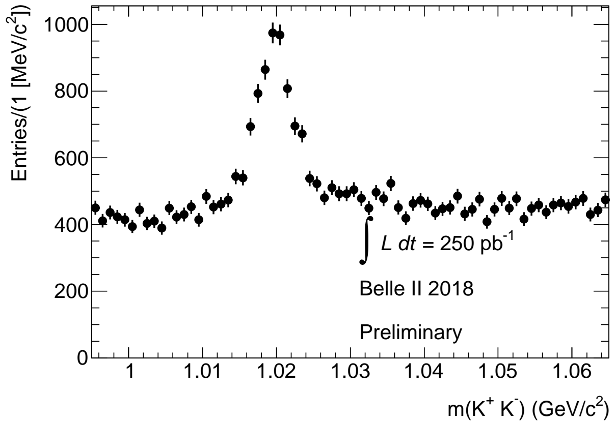
FIG. 1: This figure shows m(K^+K^-) distributions in 250 \text{ pb}^{-1} of collision data. Kaon PID requirement using all the detector is applied. The selection criteria are the same as mentioned in BELLE2-NOTE-PH-2018-005.
