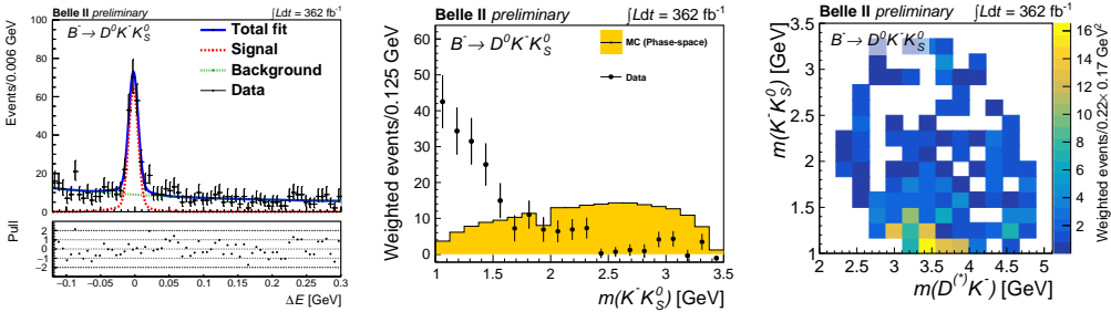
Figure 1: \Delta E distribution (left), m(K^- K_S^0) invariant mass distribution (middle) and Dalitz plot (right) of B^- \rightarrow D^0 K^- K_S^0
