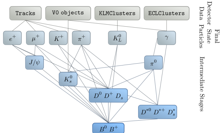
Fig. 1: Illustration of the hierarchical approach of the FEI. The graph depicts possible connections between the individual steps to reconstruct tag-side candidates in the different tag channels. Taken from [4].
