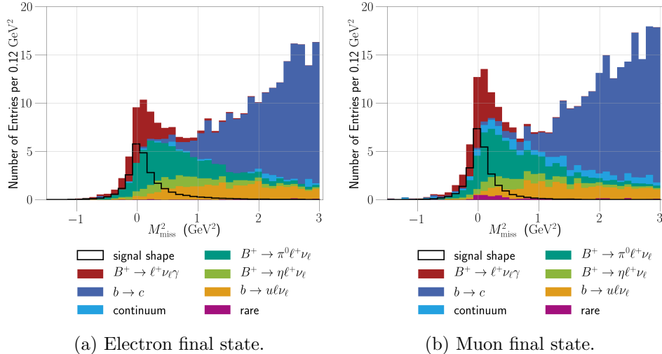
Fig. 2: Missing mass squared distributions after the final selection with a simulated partial branching fraction of \Delta\mathcal{B}(B^+ \rightarrow \ell^+ \nu_\ell \gamma) = 5.0 \times 10^{-6} .
