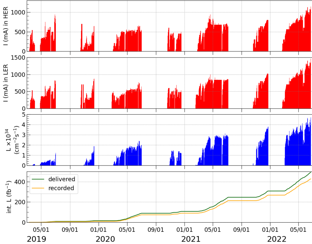
Figure 2.3: Operation history from 2019 to 2022: beam current in the HER, LER, and luminosity in a day.
