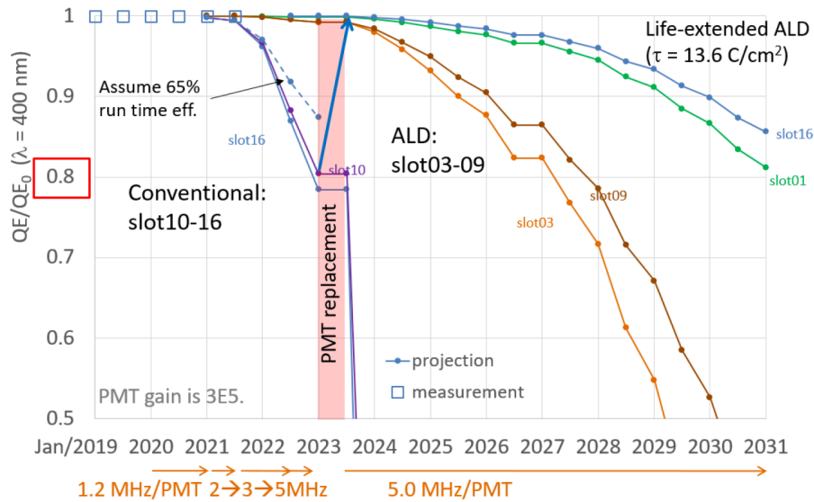
Figure 6.2: Expected projection of QE degradation for the three different generations of MCP-PMTs installed in the TOP detector: conventional, ALD and life-extended ALD. Horizontal axis shows the year and vertical axis is the relative QE.
