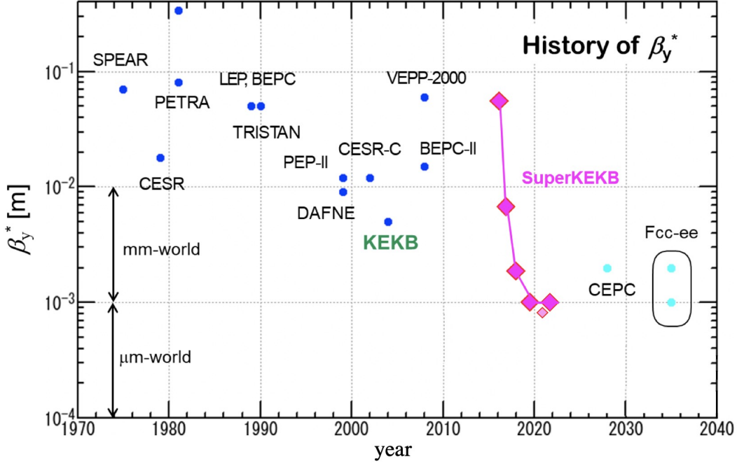
Figure 2.4: History of \beta_y^*
