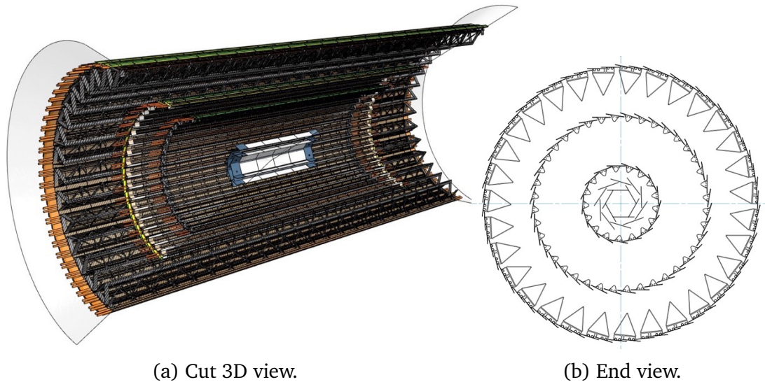
Figure 5.9: Two different views of the VTX detector layout for version 3a. The five layers are represented with their support structure, their radii are: 14 , 22 , 39 , 89 , 140 mm.
