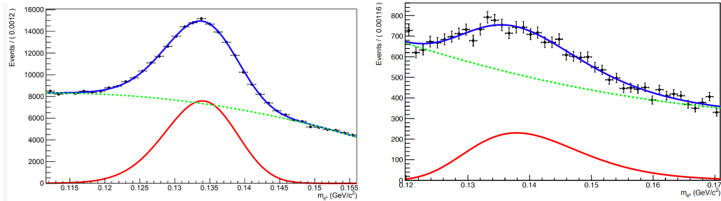
Figure 9.2: Reconstructed \pi^0 mass for the early phase-3 luminosity with BGx1 background simulation (left) and for the ultimate phase-3 BGx1 background simulation (right). The signal peak has been fitted with a Novosibirsk function while the background is described by a Chebichev distribution.
