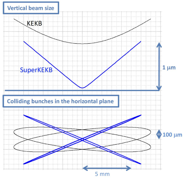
Figure 2.1: Schematic view of the nanobeam collision scheme.
