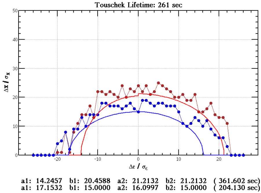
Figure 2.14: The present lattice ( \beta_y^* = 0.27 mm)
