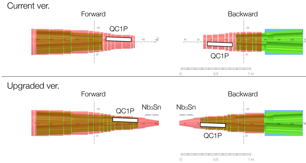
Figure 2.10: Comparison between the current QCS configuration (top) and the new QCS configuration. Anti-solenoid coils and iron (or permendur) shield are indicated in red and green, respectively.
