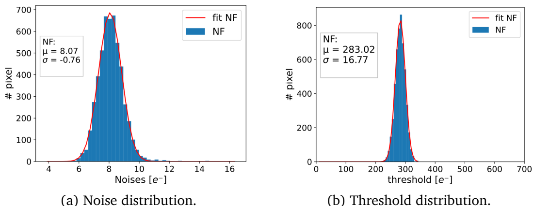
Figure 5.4: Threshold and noise distribution obtained on the normal front-end of the TJ-Monopix2 sensor, from [82].
