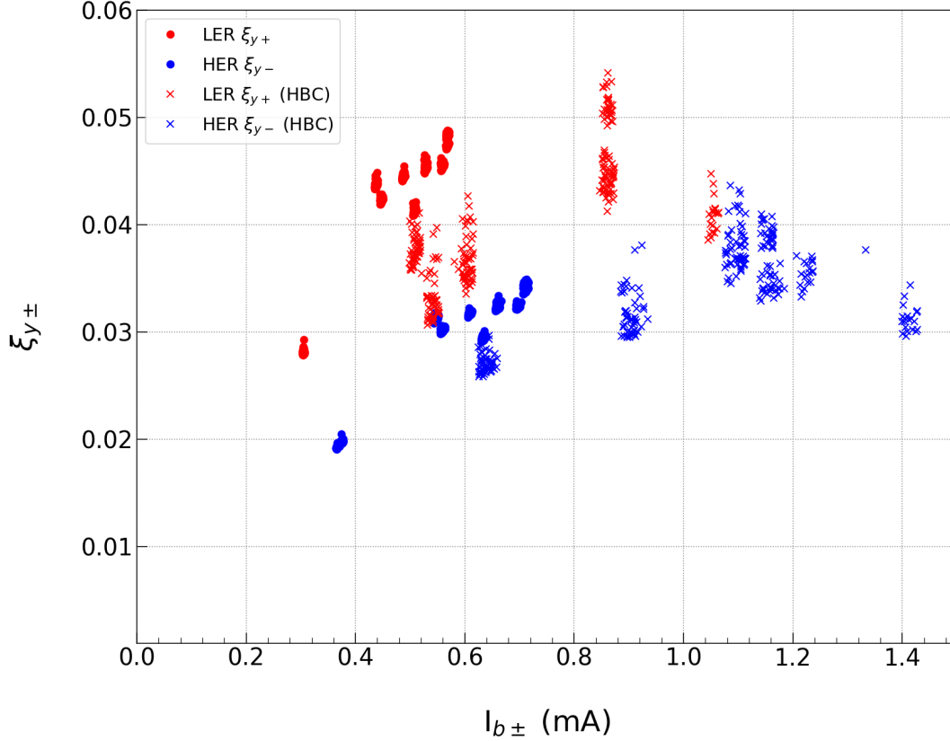
Figure 2.5: Beam–beam parameters as a function of the bunch current. The positrons in the LER are indicated by red, whereas blue is used for the electrons in the HER. The cross plots are data from the HBC.
