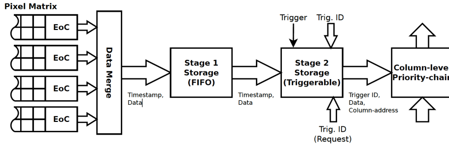
Figure 5.7: Schematic illustrating the principle of operation of the trigger logic unit (TRU).
