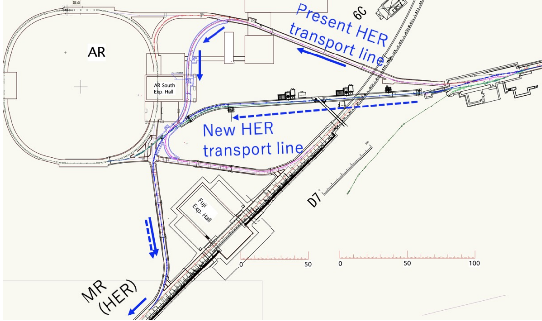
Figure 2.9: A proposed new beam transport line and the present beam transport line for the HER.
