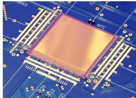
(b) Photograph of the sensor bonded on a test board.
