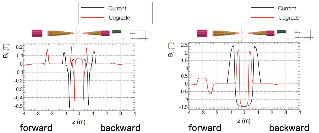
Figure 2.11: Comparison between the current and the new anti-solenoid field profile of B_x and B_z by the magnet configurations in Fig. 2.10 for the LER. Anti-solenoid coil cancels the magnetic field generated by the Belle II detector solenoid before QC1P.
