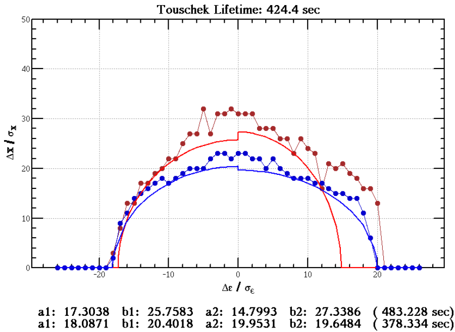
Figure 2.15: The new lattice ( \beta_y^* = 0.27 mm)
