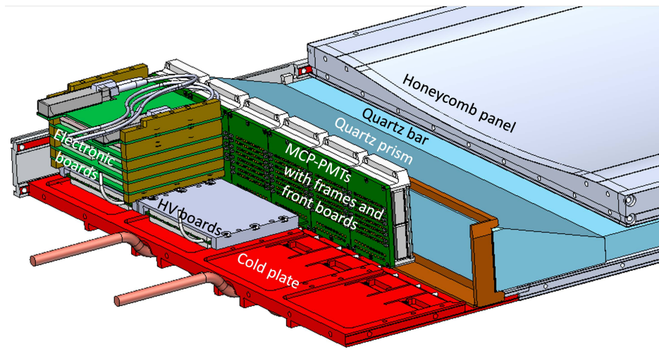
Figure 6.1: Description of the back side of one TOP module where electronic boards and photodetectors are interfaced with the quartz prism and quartz bar.
