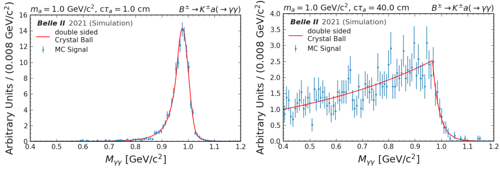
Figure 9.4: The reconstructed photon pair's invariant mass distribution in B \rightarrow Ka, a \rightarrow \gamma\gamma MC sample for the axion-like-particle (ALP), a mass m_a = 1 \text{ GeV}/c^2 , lifetime c\tau = 1 \text{ cm} (left) and 40 \text{ cm} (right) cases.
