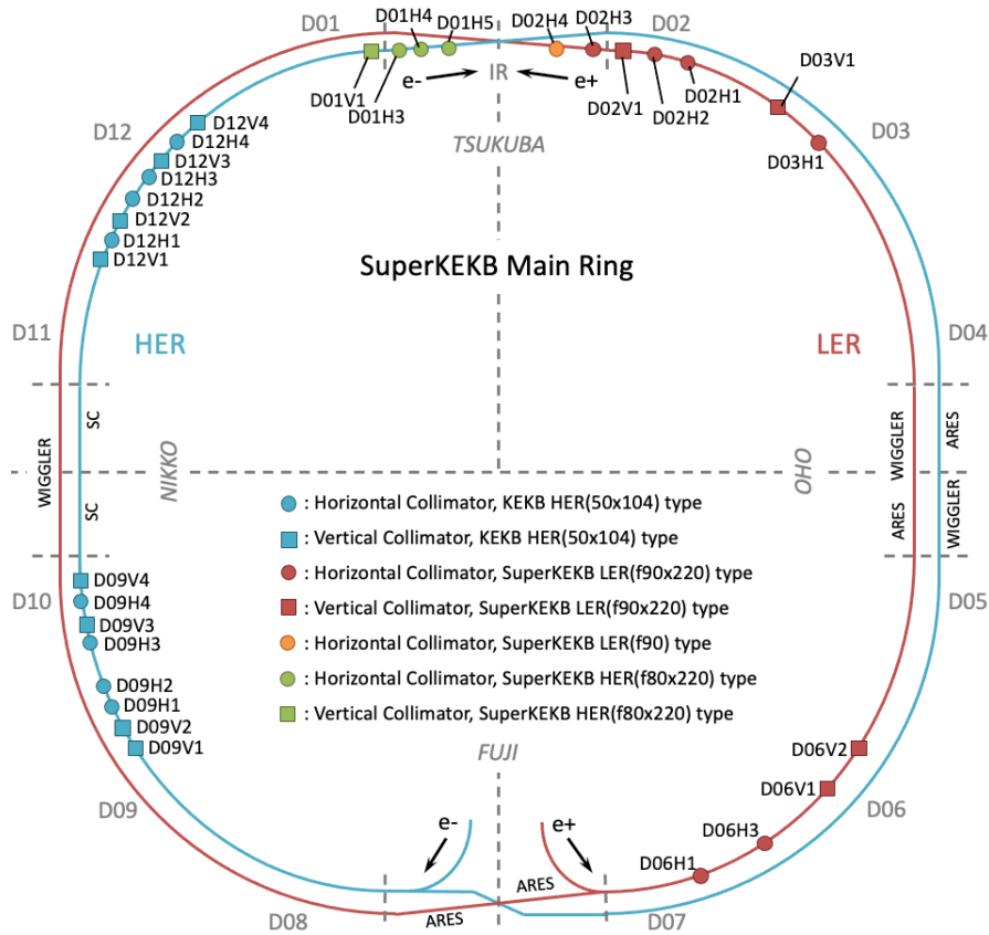
Figure 2.7: Collimator Map in 2022.
