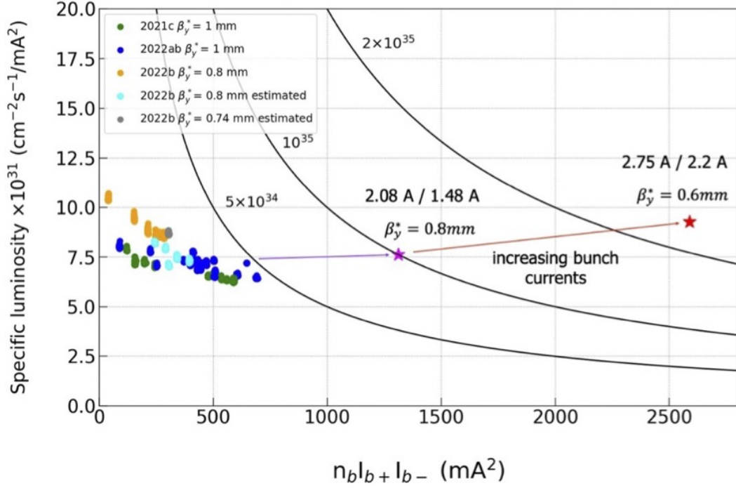
Figure 2.8: Specific luminosity plotted against the product of beam currents after LS1.
