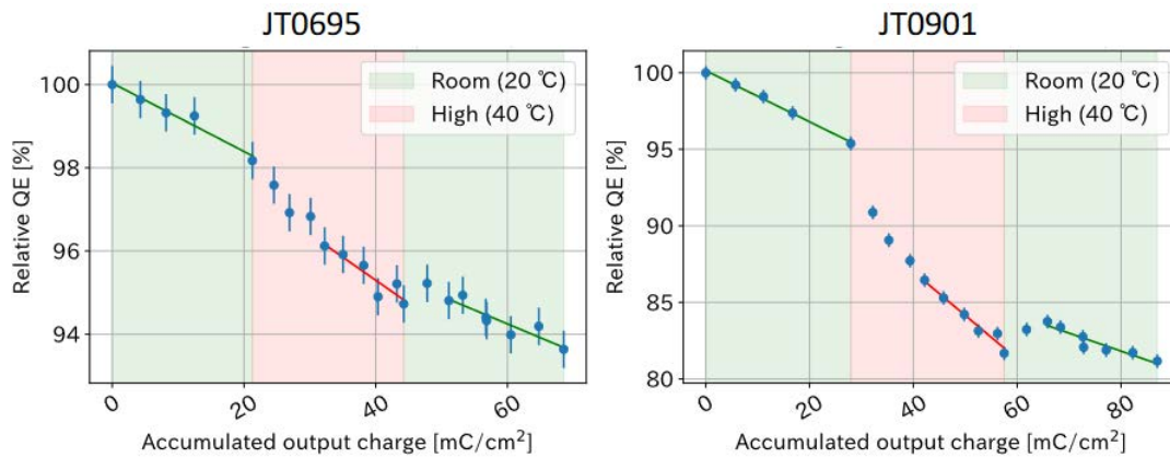
Figure 6.3: Relative QE degradation as a function of the accumulated charge at 20°C and 40°C for two MCP-PMTs.
