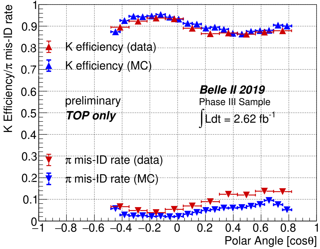
FIG. 5: Kaon efficiency and pion mis-ID rate for the TOP only PID criterion \mathcal{R}_{K/\pi} > 0.5 using the decay D^{*+} \rightarrow D^0[K^-\pi^+]\pi^+ in the bins of polar angle (laboratory frame) of the tracks.
