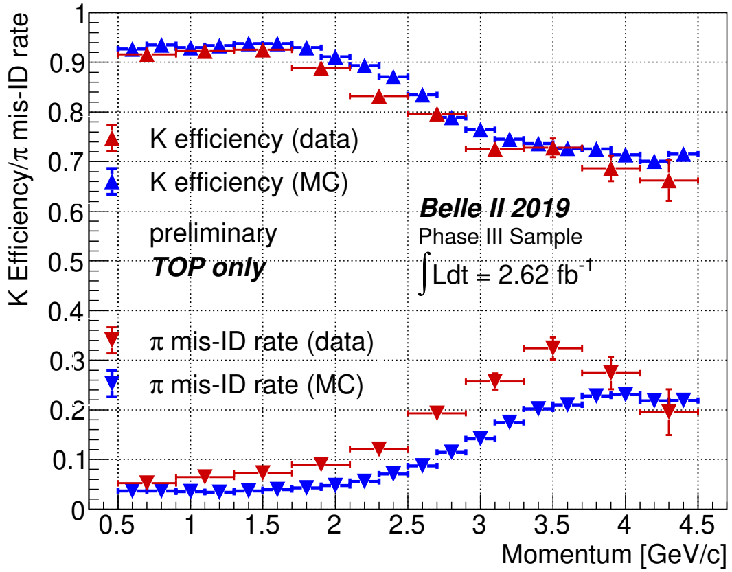
FIG. 4: Kaon efficiency and pion mis-ID rate for the TOP only PID criterion \mathcal{R}_{K/\pi} > 0.5 using the decay D^{*+} \rightarrow D^0[K^-\pi^+]\pi^+ in the bins of laboratory frame momentum of the tracks.
