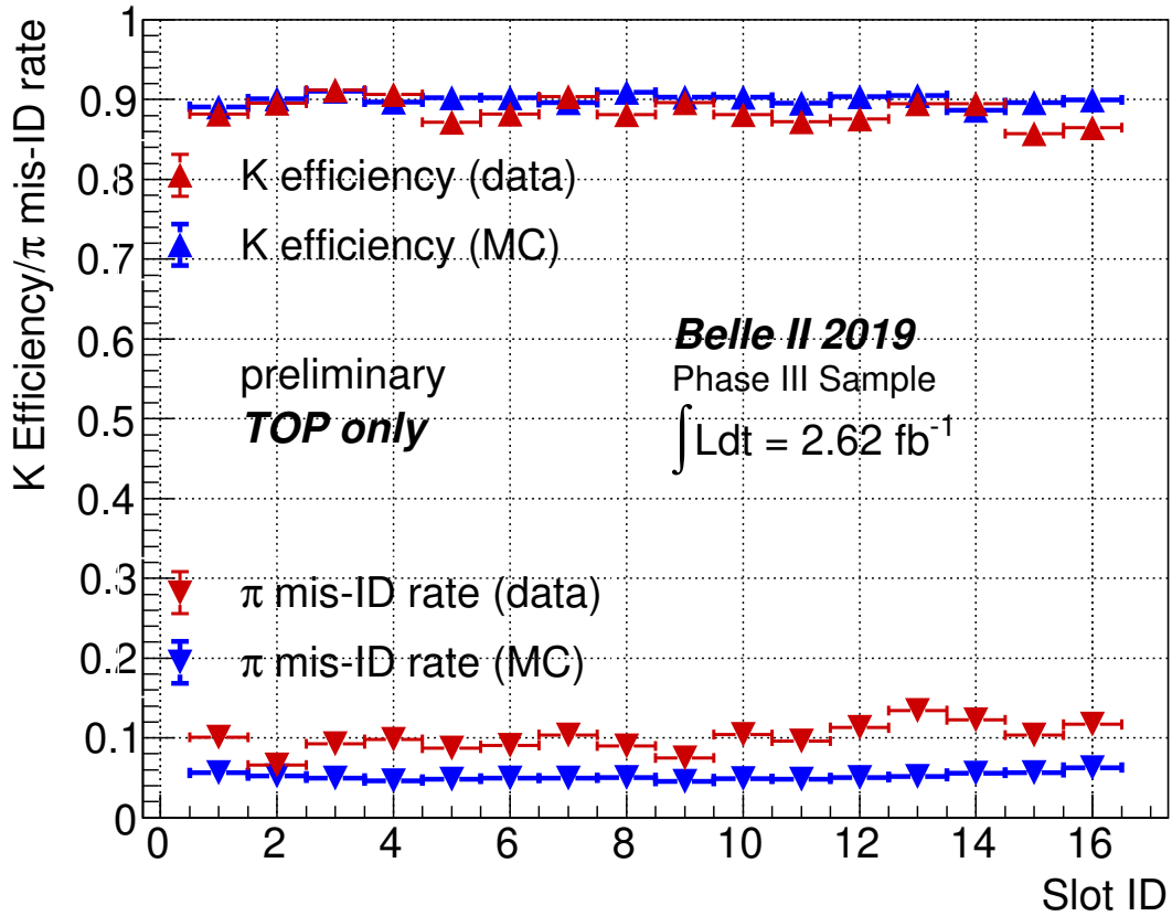
FIG. 6: Kaon efficiency and pion mis-ID rate for the TOP only PID criterion \mathcal{R}_{K/\pi} > 0.5 using the decay D^{*+} \rightarrow D^0[K^-\pi^+]\pi^+ in the 16 TOP slots (arXiv:1011.0352).
