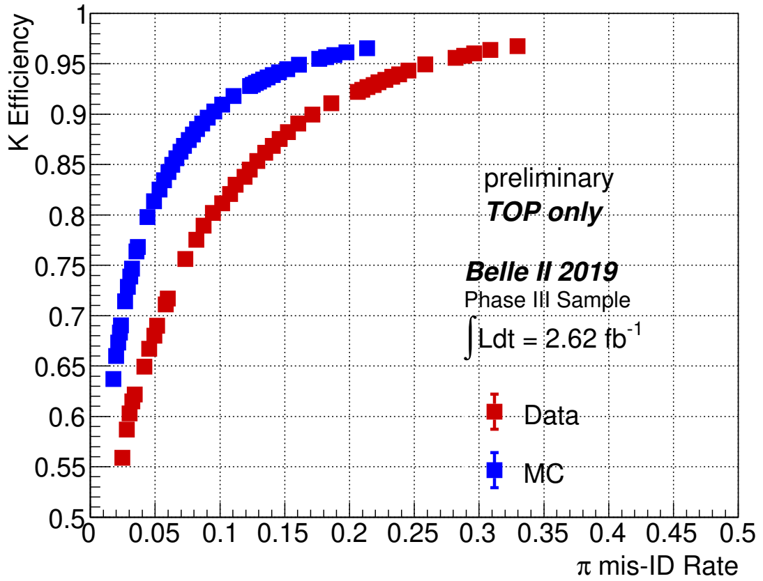
FIG. 3: TOP only K-efficiencies vs. \pi -mis-ID rates for different PID criteria using the decay D^{*+} \rightarrow D^0[K^-\pi^+]\pi^+ .
