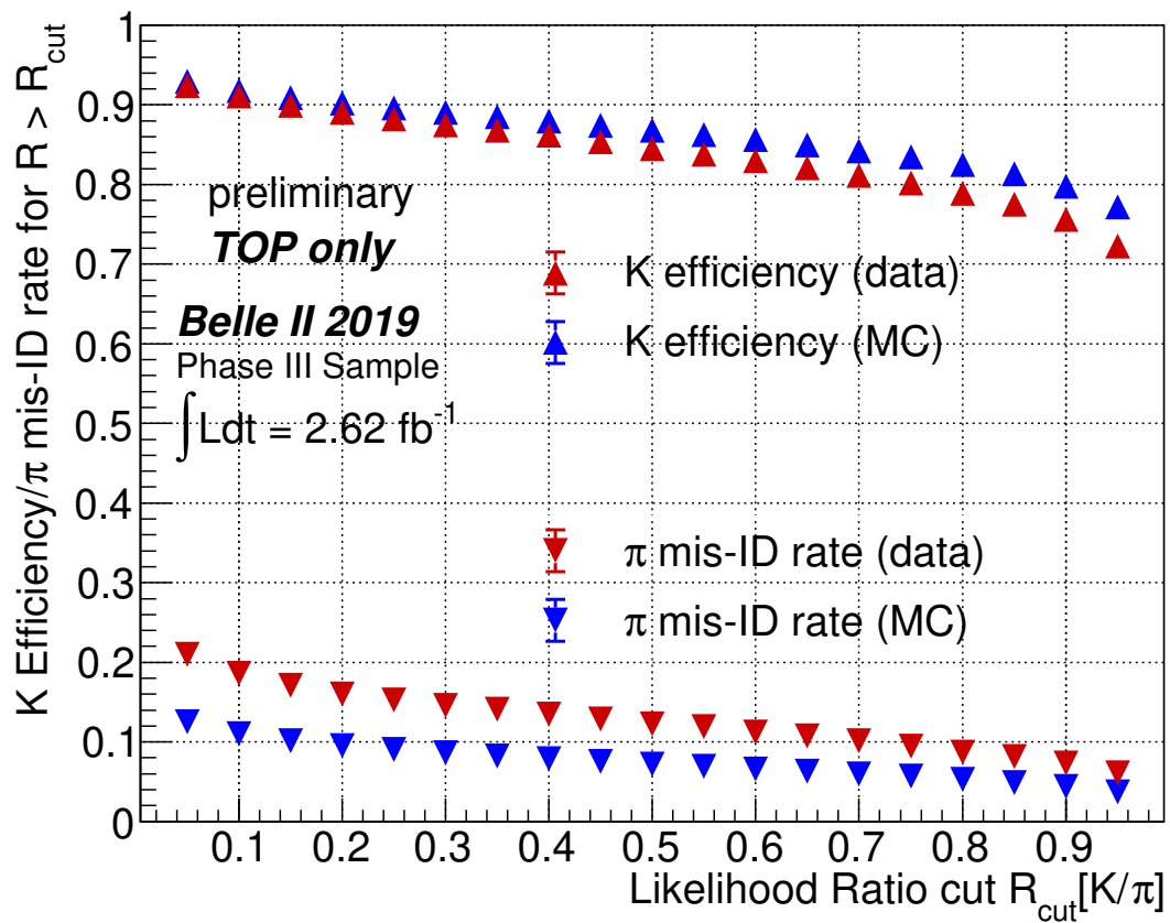
FIG. 2: TOP only K-efficiencies and \pi -mis-ID rates are calculated for different PID criteria using the decay D^{*+} \rightarrow D^0[K^-\pi^+]\pi^+ .
