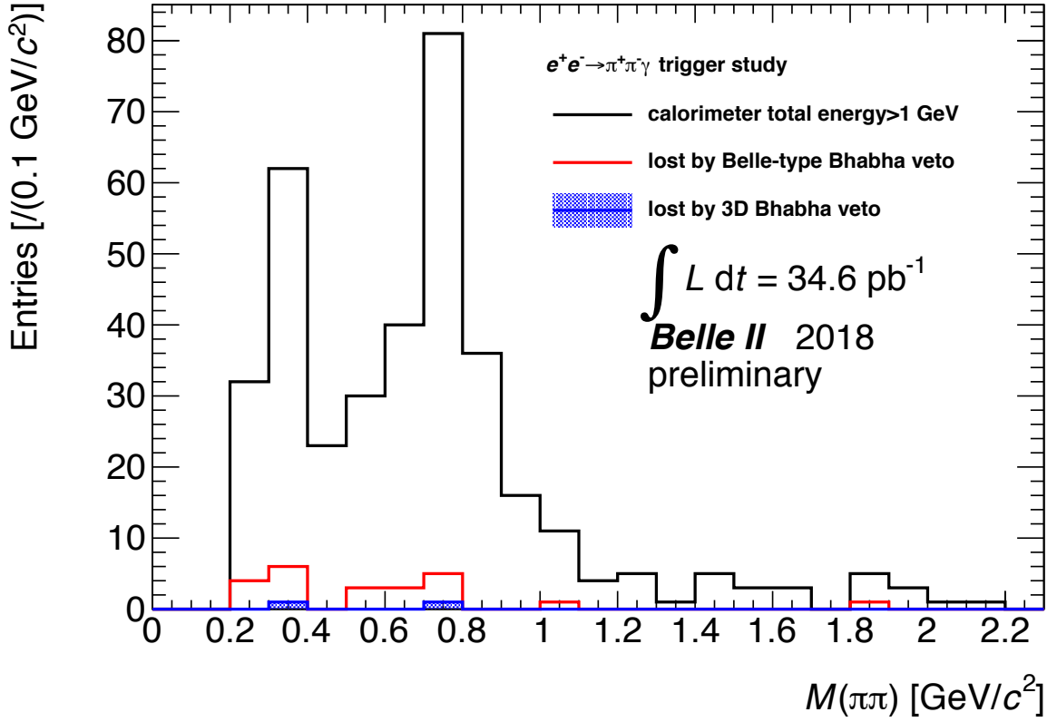
FIG. 5: This shows distribution of M(\pi\pi) with various trigger conditions for runs after the 3D Bhabha veto was implemented. To have larger statistics, limitation on ISR photon angle was loosened. The red one shows events to be lost by the Belle-type Bhabha veto and blue one by the 3D Bhabha veto. Further detail is described in BELLE2-NOTE-PH-2018-030.
