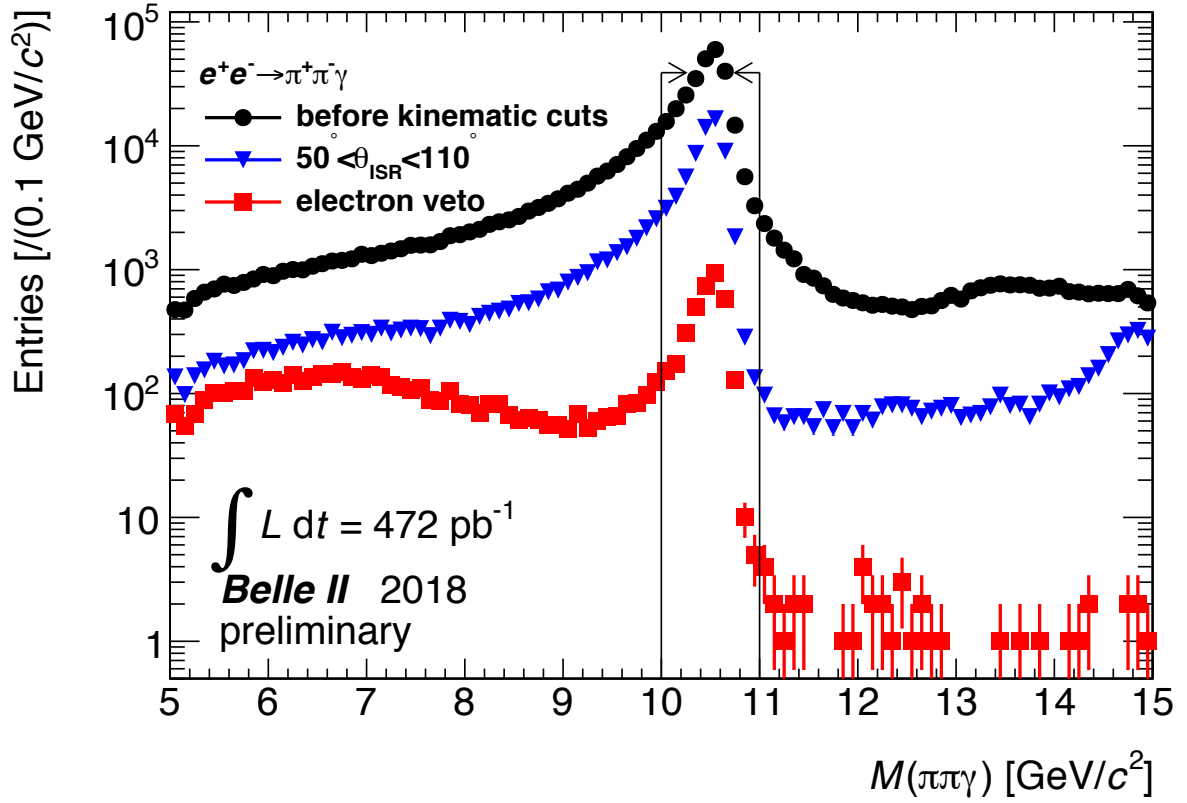
FIG. 1: This figure shows M(\pi\pi\gamma) distribution, which was produced with phase 2 full statistics. Electron veto is to reject radiative Bhabha events, and requires E/p < 0.80 for both track candidates. The peak at the collision energy indicates detection of production of two charged tracks with hard ISR from e^+e^- collision. Further detail is described in BELLE2-NOTE-PH-2018-030.
