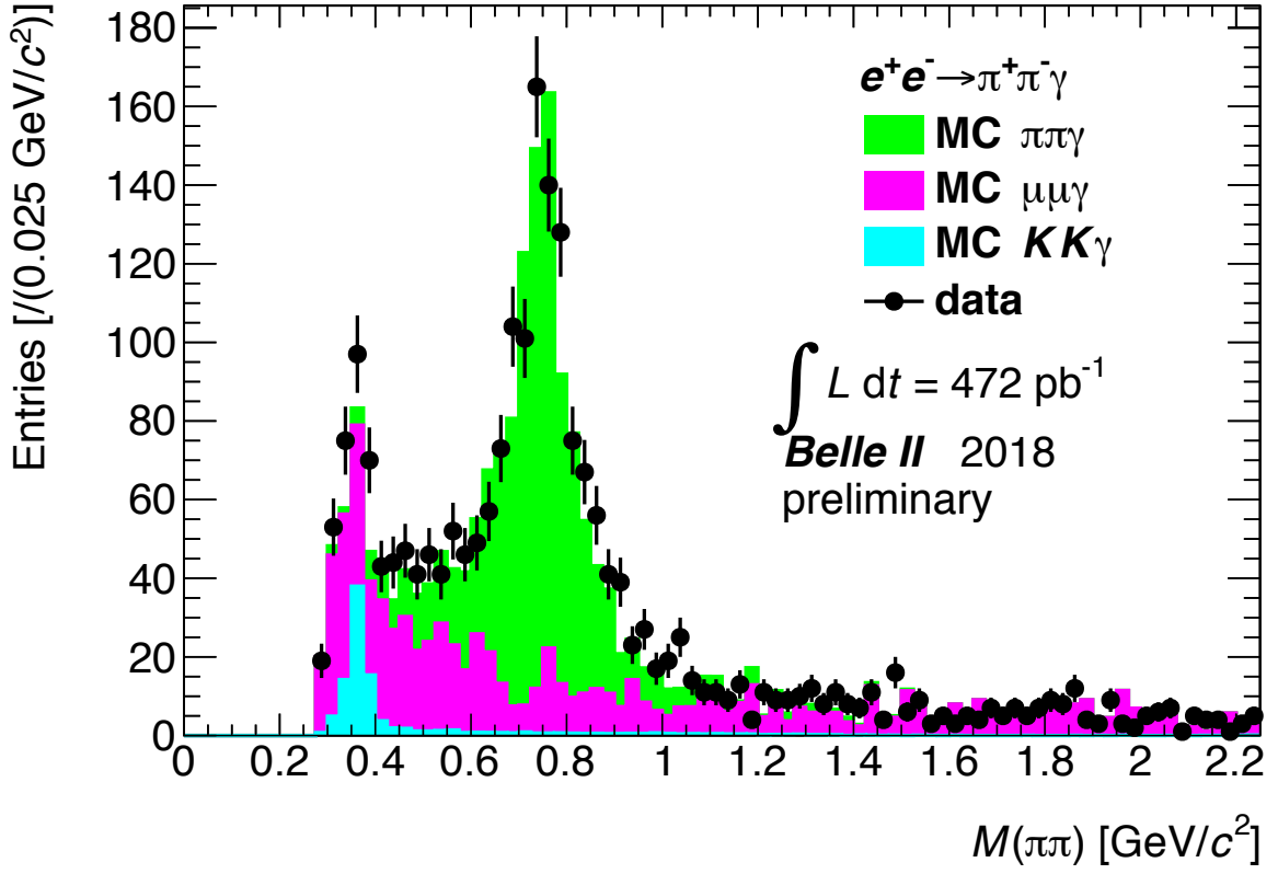
FIG. 3: This plot shows M(\pi\pi) distribution in the ee \rightarrow \pi\pi\gamma process. MC cross sections are taken from the Phokhara generator output. All the selection cuts, such as ISR photon angle, track momentum, E/p < 0.8 for electron veto. Further detail is described in BELLE2-NOTE-PH-2018-030.
