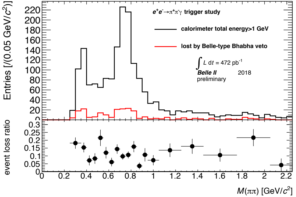
FIG. 4: This shows distribution of M(\pi\pi) with two trigger conditions. The black histogram shows events triggered by the condition of > 1 GeV total calorimeter energy deposition and the red one shows events to be lost by the Belle-type Bhabha veto. Further detail is described in BELLE2-NOTE-PH-2018-030.
