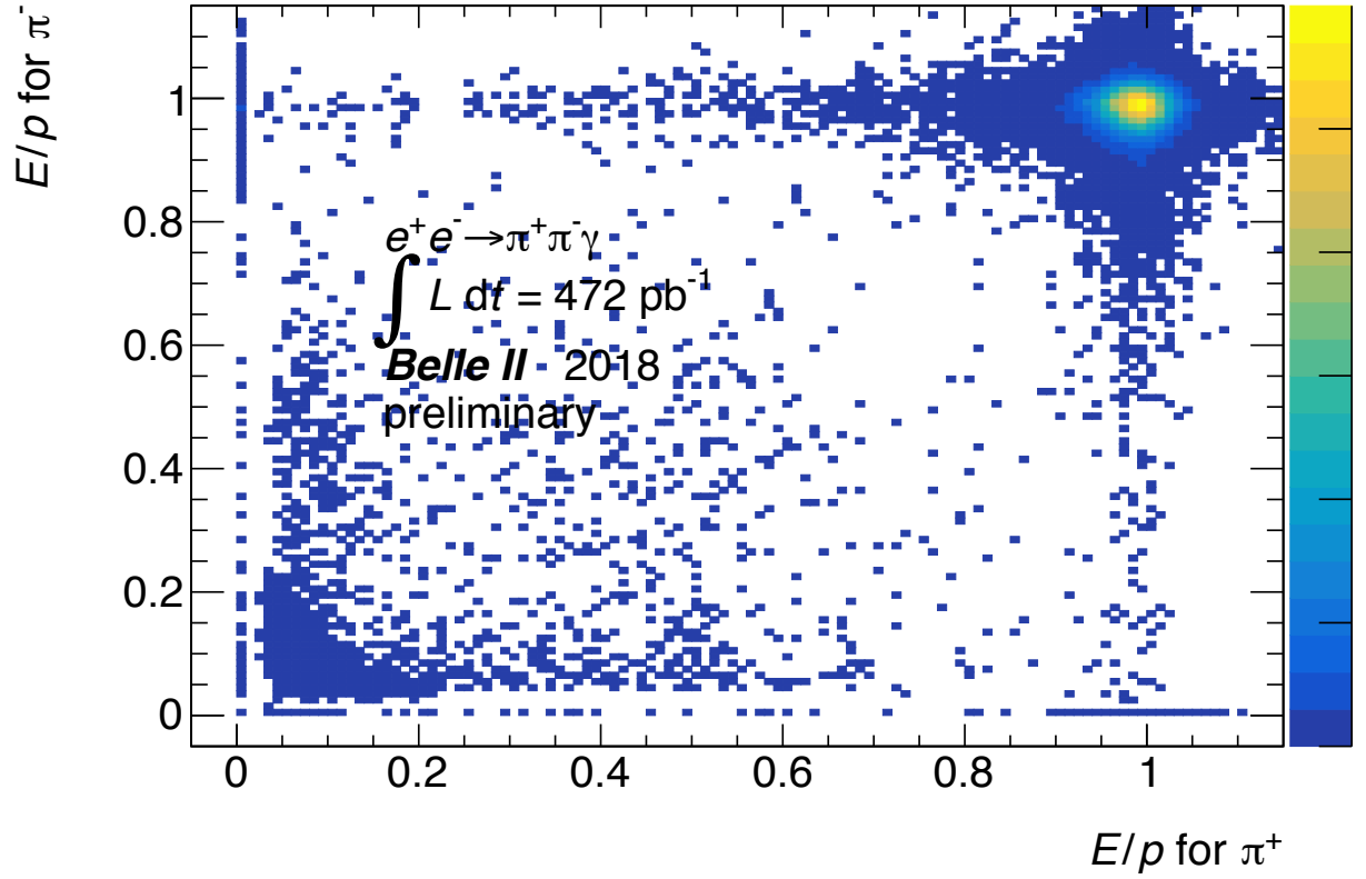
FIG. 2: This shows distribution of E/p ratio for each of positive and negative charged tracks. Most events are populated around E/p = 1 for both tracks, which indicates contribution from the radiative Bhabha process. To reject these events, E/p < 0.8 is required for both tracks. Further detail is described in BELLE2-NOTE-PH-2018-030.
