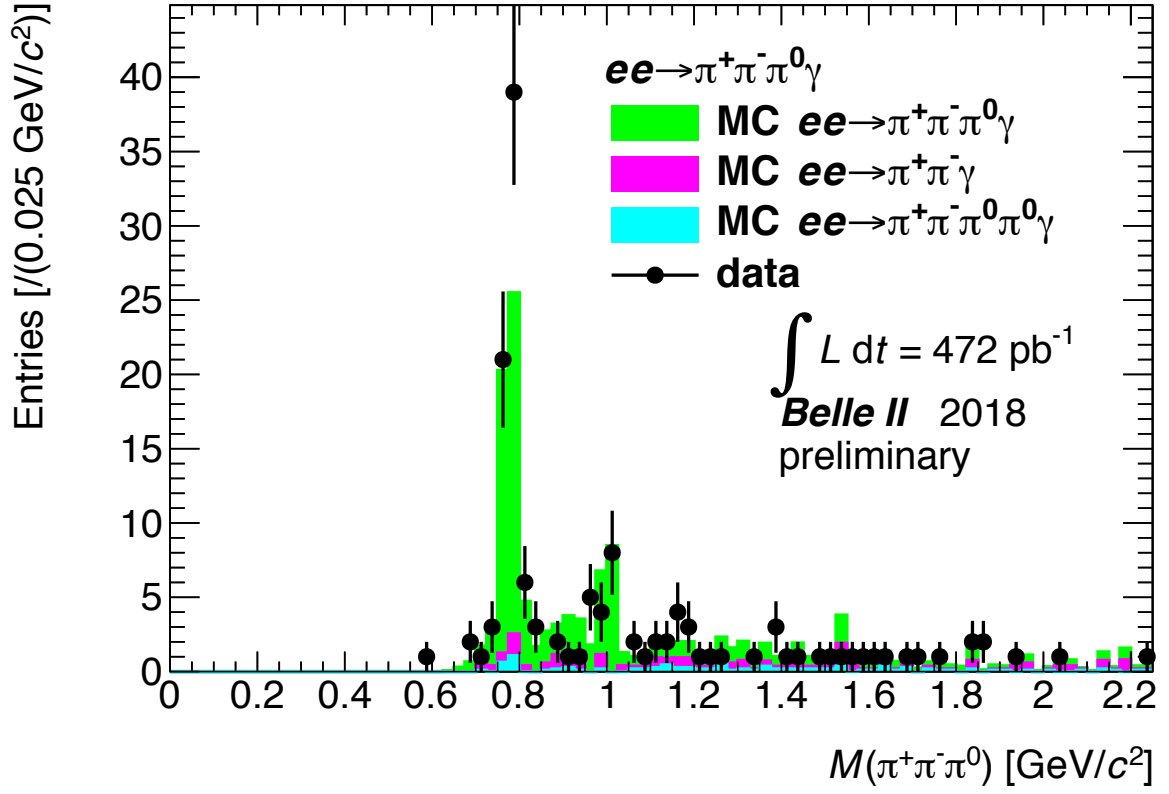
FIG. 6: This shows distribution of M(\pi^+\pi^-\pi^0) for ee \rightarrow \pi^+\pi^-\pi^0 events with the full phase2 data. Further detail is described in BELLE2-NOTE-PH-2018-030.
