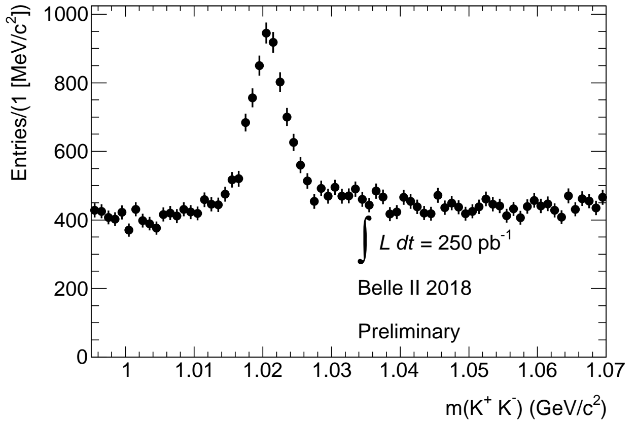
FIG. 1: This figure shows m(K^+K^-) distributions in 250 \text{ pb}^{-1} of collision data. Kaon PID requirement using all the detector is applied. The selection criteria are the same as mentioned in BELLE2-NOTE-PH-2018-005.
